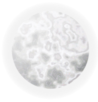
White dwarfs
